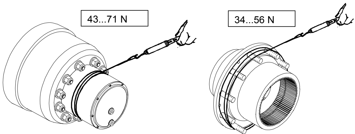
Picture 2. Rolling torque measurement with a spring scale from the wheel hub circumference.
